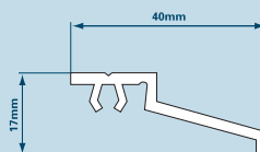
Snap On Head Drip 109.230
