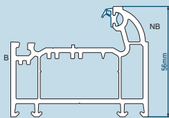
56mm Outer Frame 101.160 Steel U Channel Reinforcement 113.317
