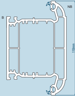
110mm Midrail 102.264 Box Steel Reinforcement 113.376 Ported Aluminium Reinforcement 115.286
