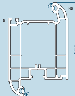
110mm Z Residential Door Sash 105.168 Box Steel Reinforcement 113.231 U Channel Steel Reinforcement 113.320 Prepared U Channel Steel Reinforcement 113.318
