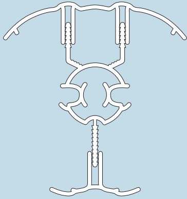
Loadbearing Variable Pole 10145
