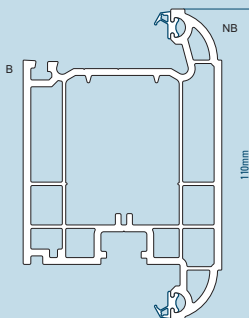
110mm T Residential Door Sash 105.169 Box Steel Reinforcement 113.231 U Channel Steel Reinforcement 113.320 Prepared U Channel Steel Reinforcement 113.318
