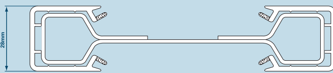
Dog Bone Coupling 113.112 Cover 116.012
