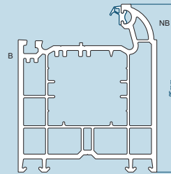
85mm Outer Frame 101.162 U Channel Steel Reinforcement 113.041 C Steel Reinforcement 113.378 Cranked Steel Reinforcement 113.371
