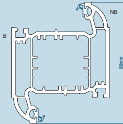
86mm Z Mullion 102.262 Box Steel Reinforcement 113.041 U Channel Steel Reinforcement 113.321 C Steel Reinforcement 113.378 Cranked Steel Reinforcement 113.371 Ported Aluminium Reinforcement 115.285
