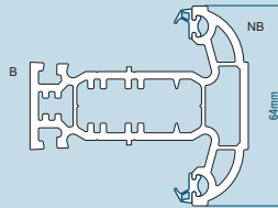
64mm T Mullion 102.261 Box Steel Reinforcement 113.041 U Channel Steel Reinforcement 113.321 Ported Aluminium Reinforcement 115.284
