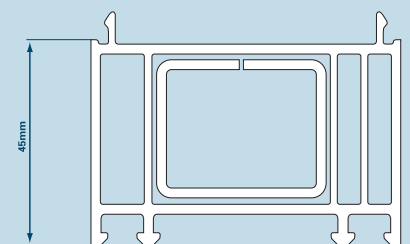
45mm frame extension 114.202 Reinforcement 113.271
