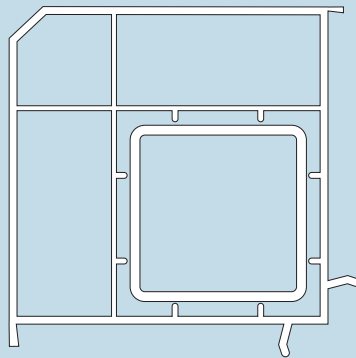
90 Degree Corner Post 116.200 Aluminium Reinforcement AL 16
