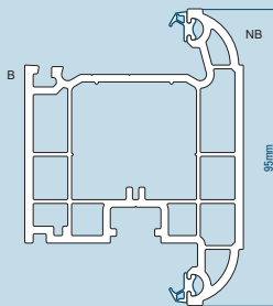
95mm T Double Door Sash 103.266 U Channel Steel Reinforcement 113.375 Prepared U Channel Steel Reinforcement 113.374
