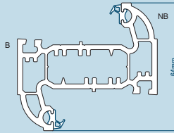
64mm Z Mullion 102.260 Box Steel Reinforcement 113.041 U Channel Steel Reinforcement 113.321 Ported Aluminium Reinforcement 115.284
