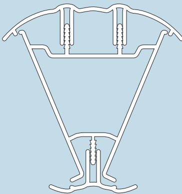
135 Degree Fixed Corner Post 10147 External Cover 10141 Internal Cover 10138
