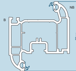
80mm Tilt & Turn Sash 103.267 Steel Reinforcement 113.373
