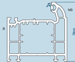
70mm Outer Frame 101.161 U Channel Steel Reinforcement 113.321 C Steel Reinforcement 113.378 Cranked Steel Reinforcement 113.371
