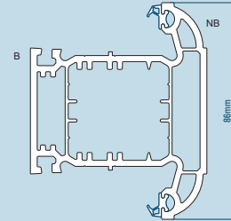
86mm T Mullion 102.263 Box Steel Reinforcement 113.041 U Channel Steel Reinforcement 113.321 C Steel Reinforcement 113.378 Cranked Steel Reinforcement 113.371 Ported Aluminium Reinforcement 115.285
