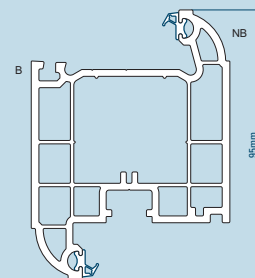
95mm Z Double Door Sash 103.265 U Channel Steel Reinforcement 113.375 Prepared U Channel Steel Reinforcement 113.374
