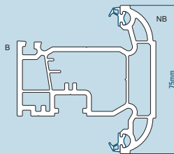
75mm Casement Sash 103.264 Steel Reinforcement 113.372
