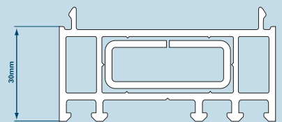
30mm frame extension 114.014 Reinforcement 113.028
